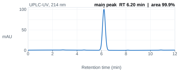
Fig. 1 — UPLC chromatogram; main peak 6.20 min, 99.9% area.
