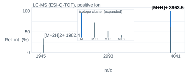
Fig. 2 — ESI-Q-TOF mass spectrum; base peak [M+H] + 3963.5 m/z.
