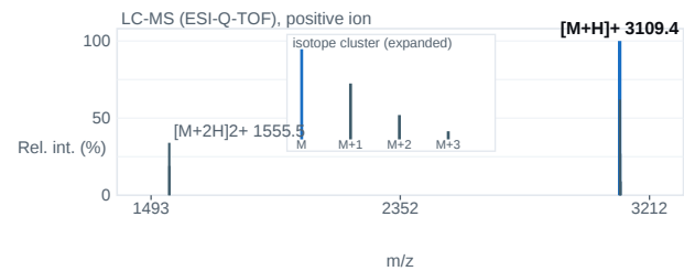
Fig. 2 — ESI-Q-TOF mass spectrum; base peak [M+H] + 3109.4 m/z.
