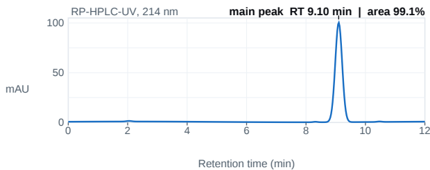
Fig. 1 — HPLC chromatogram; main peak 9.10 min, 99.1% area.
