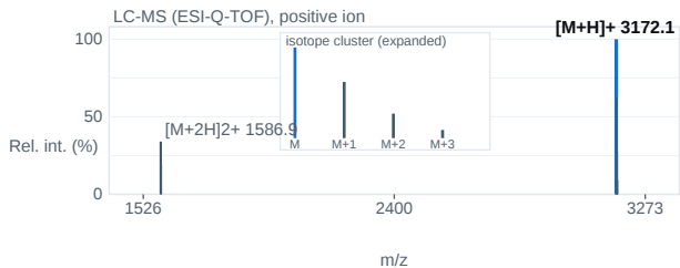
Fig. 2 — ESI-Q-TOF mass spectrum; base peak [M+H] + 3172.1 m/z.
