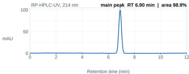
Fig. 1 — HPLC chromatogram; main peak 6.90 min, 98.9% area.
