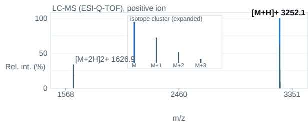
Fig. 2 — ESI-Q-TOF mass spectrum; base peak [M+H] + 3252.1 m/z.
