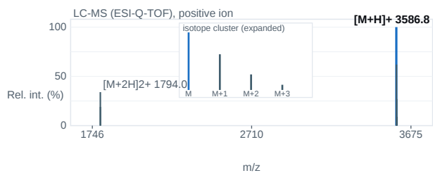
Fig. 2 — ESI-Q-TOF mass spectrum; base peak [M+H] + 3586.8 m/z.
