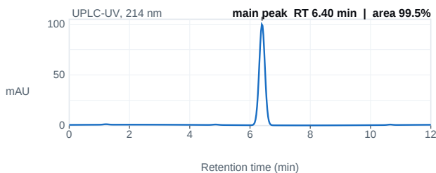
Fig. 1 — UPLC chromatogram; main peak 6.40 min, 99.5% area.
