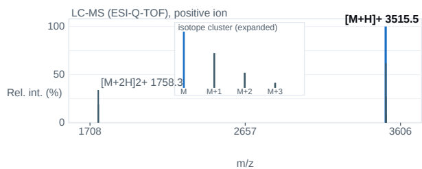
Fig. 2 — ESI-Q-TOF mass spectrum; base peak [M+H] + 3515.5 m/z.
