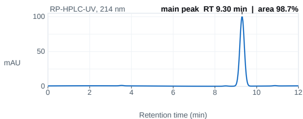
Fig. 1 — HPLC chromatogram; main peak 9.30 min, 98.7% area.
