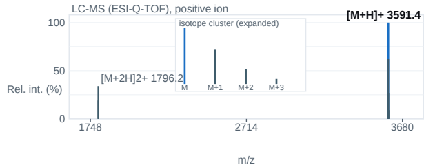
Fig. 2 — ESI-Q-TOF mass spectrum; base peak [M+H] + 3591.4 m/z.
