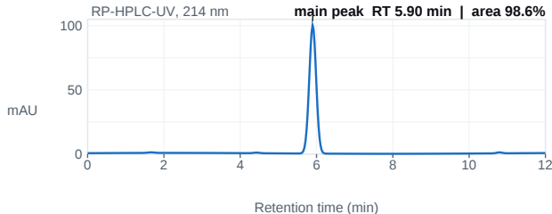
Fig. 1 — HPLC chromatogram; main peak 5.90 min, 98.6% area.
