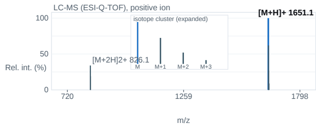
Fig. 2 — ESI-Q-TOF mass spectrum; base peak [M+H] + 1651.1 m/z.
