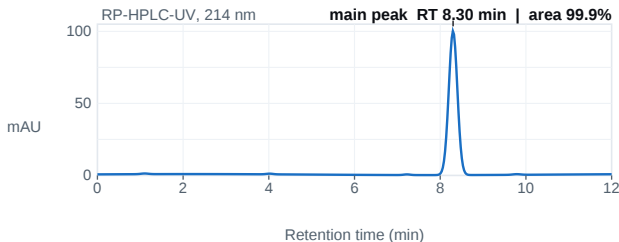
Fig. 1 — HPLC chromatogram; main peak 8.30 min, 99.9% area.
