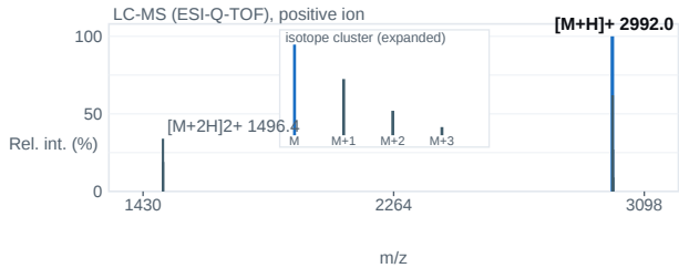
Fig. 2 — ESI-Q-TOF mass spectrum; base peak [M+H] + 2992.0 m/z.
