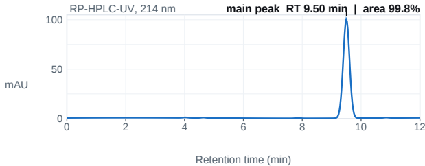
Fig. 1 — HPLC chromatogram; main peak 9.50 min, 99.8% area.
