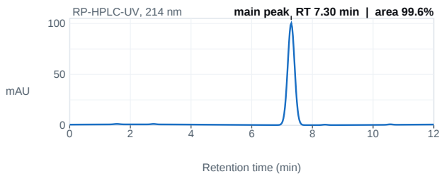
Fig. 1 — HPLC chromatogram; main peak 7.30 min, 99.6% area.
