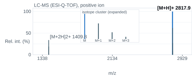
Fig. 2 — ESI-Q-TOF mass spectrum; base peak [M+H] + 2817.9 m/z.
