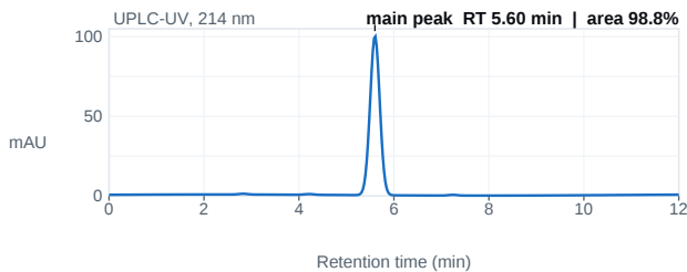
Fig. 1 — UPLC chromatogram; main peak 5.60 min, 98.8% area.
