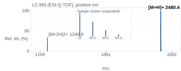
Fig. 2 — ESI-Q-TOF mass spectrum; base peak [M+H] + 2480.4 m/z.
