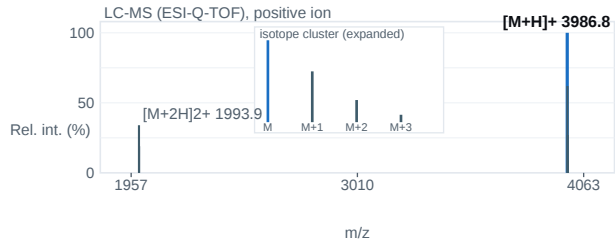
Fig. 2 — ESI-Q-TOF mass spectrum; base peak [M+H] + 3986.8 m/z.
