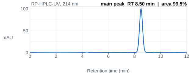
Fig. 1 — HPLC chromatogram; main peak 8.50 min, 99.5% area.
