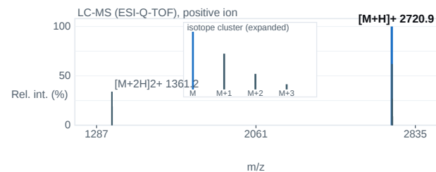
Fig. 2 — ESI-Q-TOF mass spectrum; base peak [M+H] + 2720.9 m/z.
