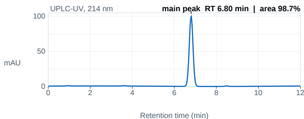
Fig. 1 — UPLC chromatogram; main peak 6.80 min, 98.7% area.
