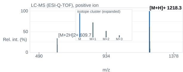
Fig. 2 — ESI-Q-TOF mass spectrum; base peak [M+H] + 1218.3 m/z.
