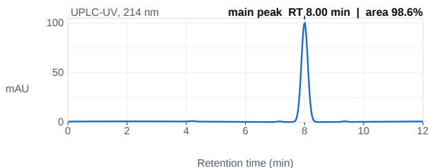
Fig. 1 — UPLC chromatogram; main peak 8.00 min, 98.6% area.
