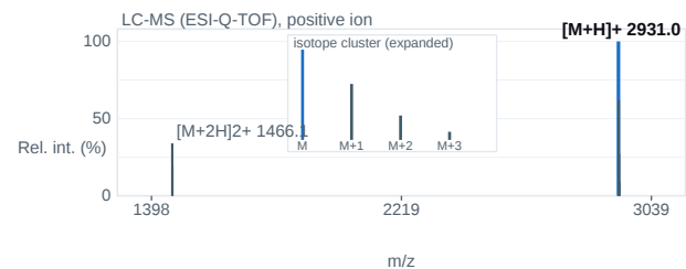
Fig. 2 — ESI-Q-TOF mass spectrum; base peak [M+H] + 2931.0 m/z.
