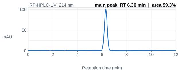
Fig. 1 — HPLC chromatogram; main peak 6.30 min, 99.3% area.
