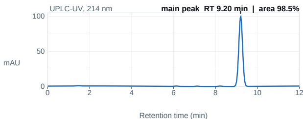
Fig. 1 — UPLC chromatogram; main peak 9.20 min, 98.5% area.
