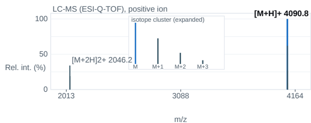
Fig. 2 — ESI-Q-TOF mass spectrum; base peak [M+H] + 4090.8 m/z.
