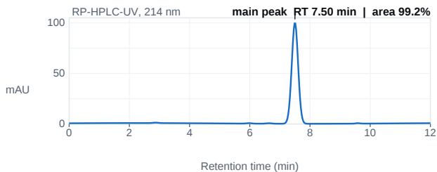
Fig. 1 — HPLC chromatogram; main peak 7.50 min, 99.2% area.
