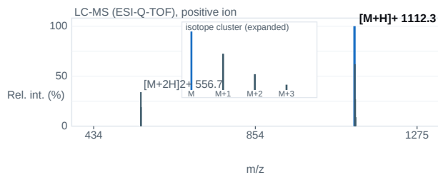
Fig. 2 — ESI-Q-TOF mass spectrum; base peak [M+H] + 1112.3 m/z.
