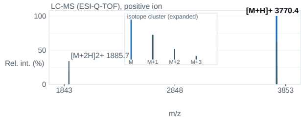
Fig. 2 — ESI-Q-TOF mass spectrum; base peak [M+H] + 3770.4 m/z.
