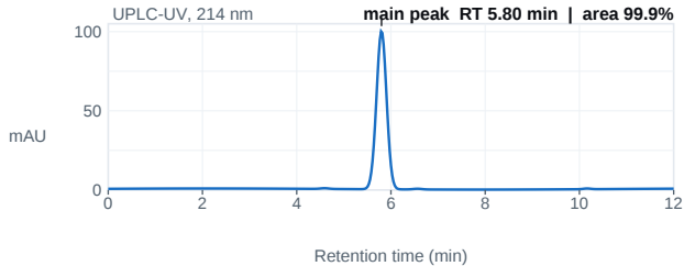
Fig. 1 — UPLC chromatogram; main peak 5.80 min, 99.9% area.
