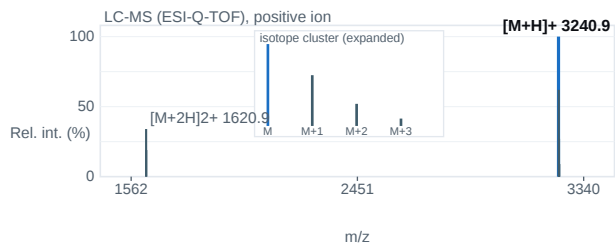
Fig. 2 — ESI-Q-TOF mass spectrum; base peak [M+H] + 3240.9 m/z.
