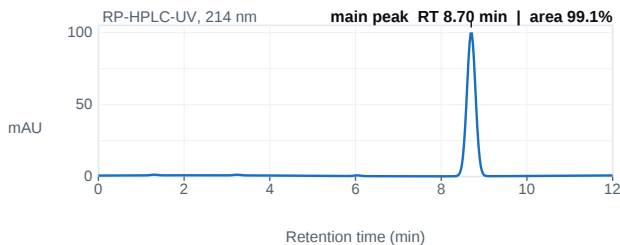
Fig. 1 — HPLC chromatogram; main peak 8.70 min, 99.1% area.
