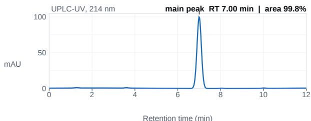
Fig. 1 — UPLC chromatogram; main peak 7.00 min, 99.8% area.
