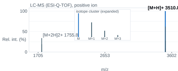
Fig. 2 — ESI-Q-TOF mass spectrum; base peak [M+H] + 3510.8 m/z.
