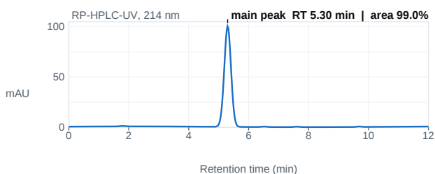
Fig. 1 — HPLC chromatogram; main peak 5.30 min, 99.0% area.
