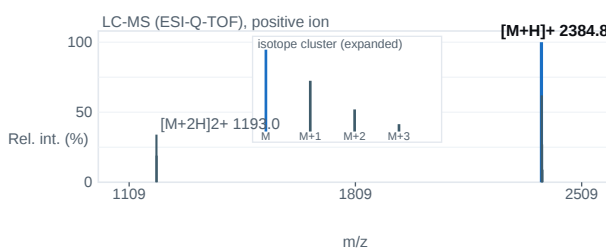
Fig. 2 — ESI-Q-TOF mass spectrum; base peak [M+H] + 2384.8 m/z.
