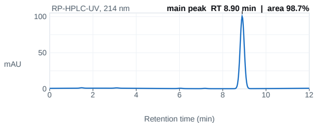
Fig. 1 — HPLC chromatogram; main peak 8.90 min, 98.7% area.
