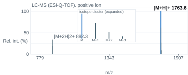
Fig. 2 — ESI-Q-TOF mass spectrum; base peak [M+H] + 1763.6 m/z.
