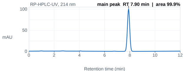
Fig. 1 — HPLC chromatogram; main peak 7.90 min, 99.9% area.
