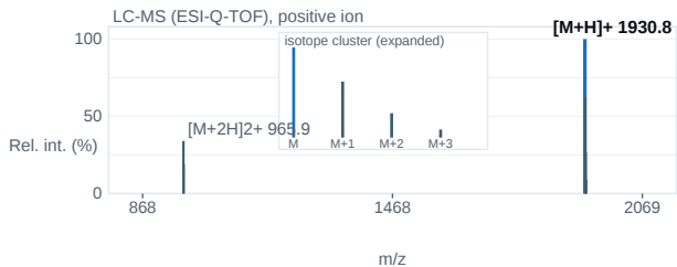
Fig. 2 — ESI-Q-TOF mass spectrum; base peak [M+H] + 1930.8 m/z.
