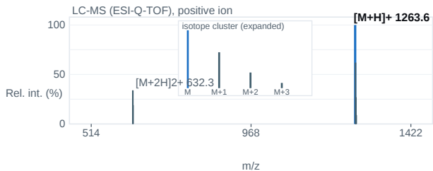
Fig. 2 — ESI-Q-TOF mass spectrum; base peak [M+H] + 1263.6 m/z.
