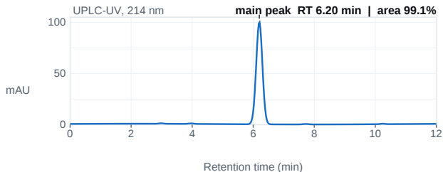
Fig. 1 — UPLC chromatogram; main peak 6.20 min, 99.1% area.
