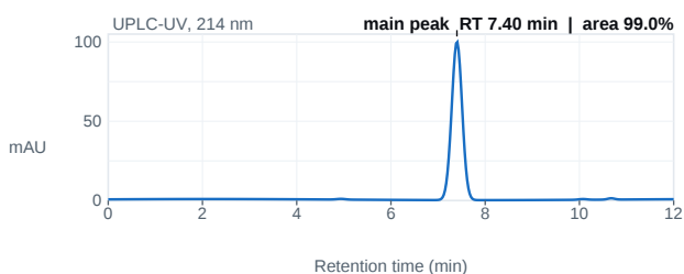
Fig. 1 — UPLC chromatogram; main peak 7.40 min, 99.0% area.
