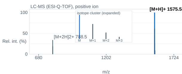
Fig. 2 — ESI-Q-TOF mass spectrum; base peak [M+H] + 1575.5 m/z.
