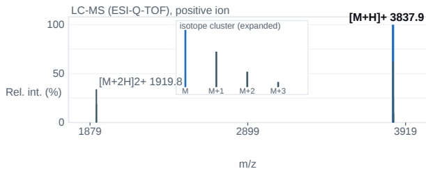
Fig. 2 — ESI-Q-TOF mass spectrum; base peak [M+H] + 3837.9 m/z.
