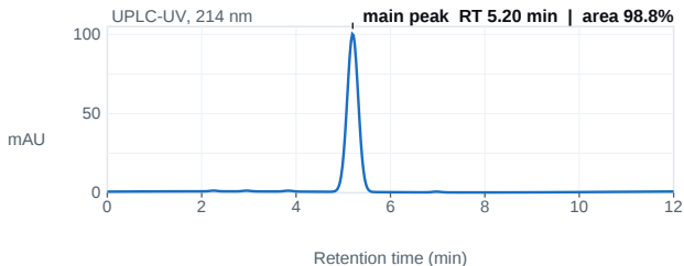
Fig. 1 — UPLC chromatogram; main peak 5.20 min, 98.8% area.
