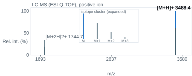
Fig. 2 — ESI-Q-TOF mass spectrum; base peak [M+H] + 3488.4 m/z.
