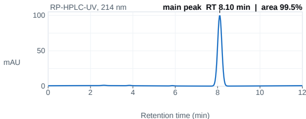
Fig. 1 — HPLC chromatogram; main peak 8.10 min, 99.5% area.
