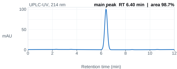
Fig. 1 — UPLC chromatogram; main peak 6.40 min, 98.7% area.
