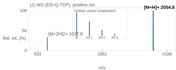
Fig. 2 — ESI-Q-TOF mass spectrum; base peak [M+H] + 2054.8 m/z.
