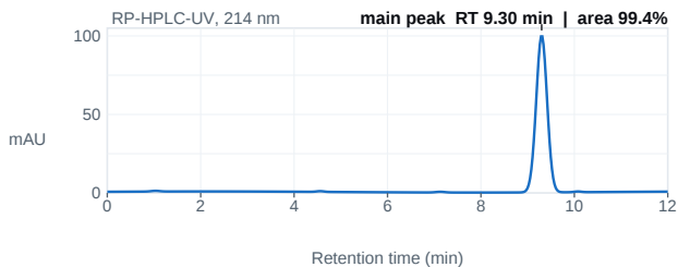
Fig. 1 — HPLC chromatogram; main peak 9.30 min, 99.4% area.
