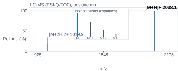
Fig. 2 — ESI-Q-TOF mass spectrum; base peak [M+H] + 2038.1 m/z.
