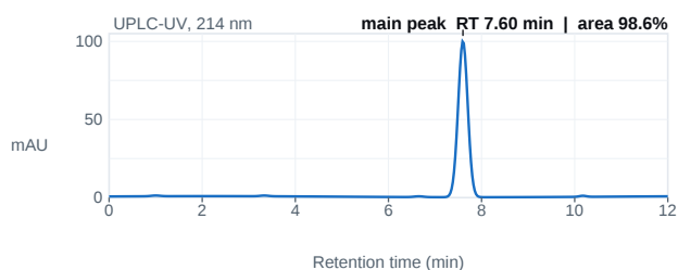
Fig. 1 — UPLC chromatogram; main peak 7.60 min, 98.6% area.
