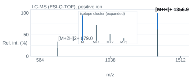
Fig. 2 — ESI-Q-TOF mass spectrum; base peak [M+H] + 1356.9 m/z.
