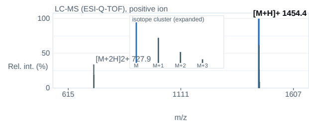
Fig. 2 — ESI-Q-TOF mass spectrum; base peak [M+H] + 1454.4 m/z.
