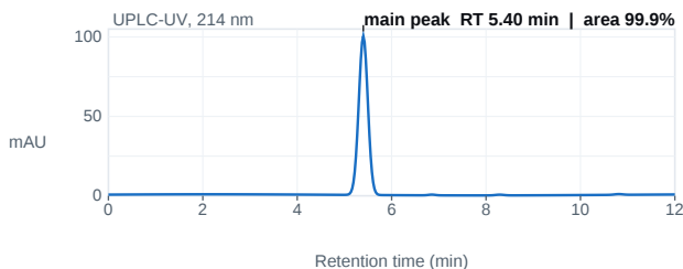
Fig. 1 — UPLC chromatogram; main peak 5.40 min, 99.9% area.
