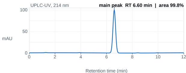
Fig. 1 — UPLC chromatogram; main peak 6.60 min, 99.8% area.
