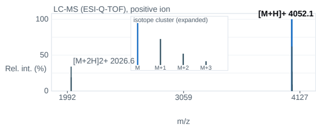
Fig. 2 — ESI-Q-TOF mass spectrum; base peak [M+H] + 4052.1 m/z.
