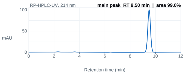
Fig. 1 — HPLC chromatogram; main peak 9.50 min, 99.0% area.
