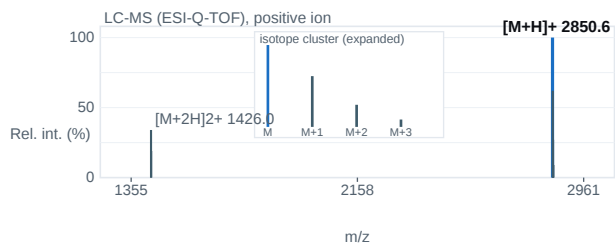
Fig. 2 — ESI-Q-TOF mass spectrum; base peak [M+H] + 2850.6 m/z.
