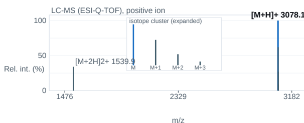
Fig. 2 — ESI-Q-TOF mass spectrum; base peak [M+H] + 3078.1 m/z.
