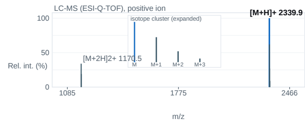
Fig. 2 — ESI-Q-TOF mass spectrum; base peak [M+H] + 2339.9 m/z.
