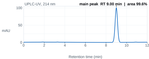
Fig. 1 — UPLC chromatogram; main peak 9.00 min, 99.6% area.
