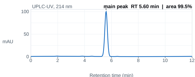
Fig. 1 — UPLC chromatogram; main peak 5.60 min, 99.5% area.
