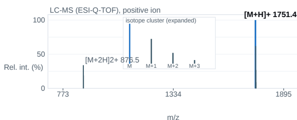
Fig. 2 — ESI-Q-TOF mass spectrum; base peak [M+H] + 1751.4 m/z.
