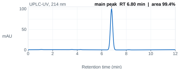
Fig. 1 — UPLC chromatogram; main peak 6.80 min, 99.4% area.
