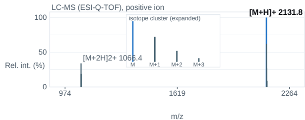
Fig. 2 — ESI-Q-TOF mass spectrum; base peak [M+H] + 2131.8 m/z.
