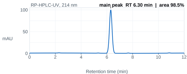
Fig. 1 — HPLC chromatogram; main peak 6.30 min, 98.5% area.
