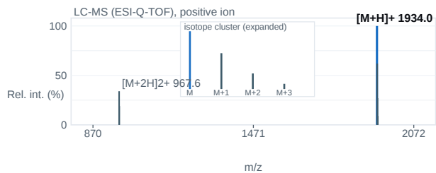
Fig. 2 — ESI-Q-TOF mass spectrum; base peak [M+H] + 1934.0 m/z.
