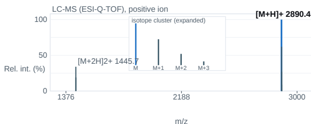
Fig. 2 — ESI-Q-TOF mass spectrum; base peak [M+H] + 2890.4 m/z.
