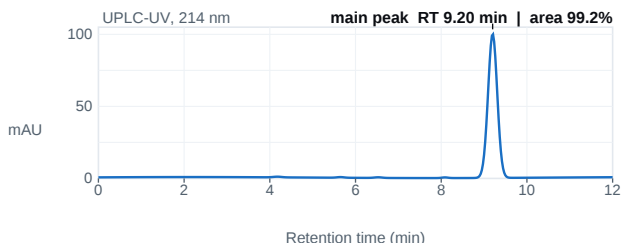
Fig. 1 — UPLC chromatogram; main peak 9.20 min, 99.2% area.
