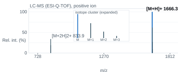
Fig. 2 — ESI-Q-TOF mass spectrum; base peak [M+H] + 1666.3 m/z.
