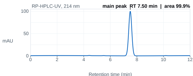
Fig. 1 — HPLC chromatogram; main peak 7.50 min, 99.9% area.
