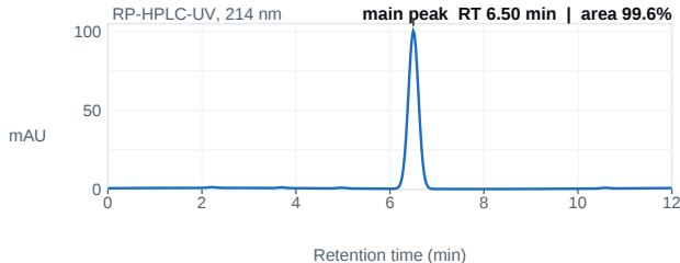
Fig. 1 — HPLC chromatogram; main peak 6.50 min, 99.6% area.
