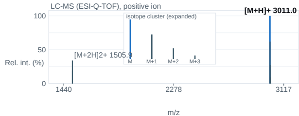
Fig. 2 — ESI-Q-TOF mass spectrum; base peak [M+H] + 3011.0 m/z.
