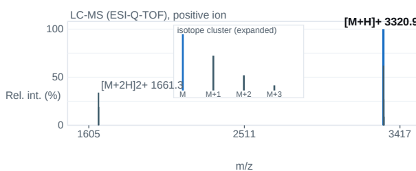
Fig. 2 — ESI-Q-TOF mass spectrum; base peak [M+H] + 3320.9 m/z.
