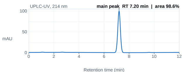
Fig. 1 — UPLC chromatogram; main peak 7.20 min, 98.6% area.
