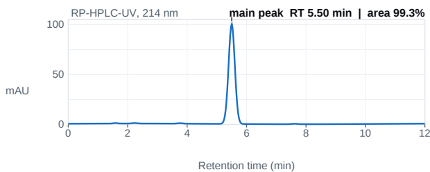
Fig. 1 — HPLC chromatogram; main peak 5.50 min, 99.3% area.
