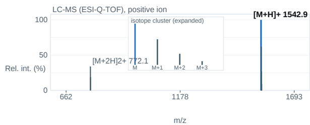
Fig. 2 — ESI-Q-TOF mass spectrum; base peak [M+H] + 1542.9 m/z.
