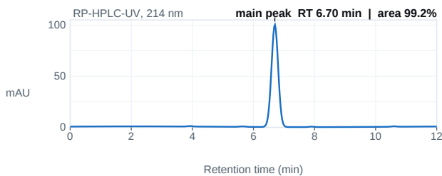
Fig. 1 — HPLC chromatogram; main peak 6.70 min, 99.2% area.
