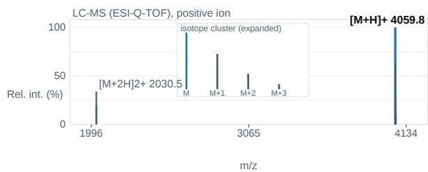
Fig. 2 — ESI-Q-TOF mass spectrum; base peak [M+H] + 4059.8 m/z.
