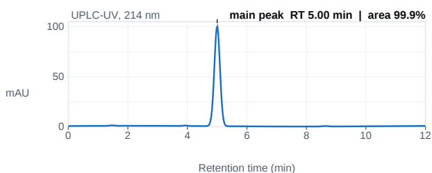
Fig. 1 — UPLC chromatogram; main peak 5.00 min, 99.9% area.
