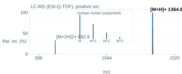
Fig. 2 — ESI-Q-TOF mass spectrum; base peak [M+H] + 1364.8 m/z.
