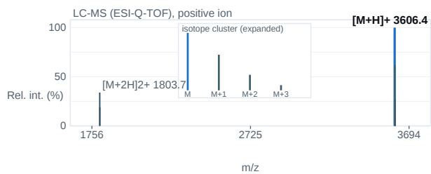
Fig. 2 — ESI-Q-TOF mass spectrum; base peak [M+H] + 3606.4 m/z.
