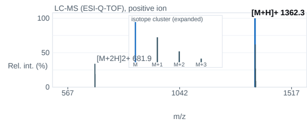
Fig. 2 — ESI-Q-TOF mass spectrum; base peak [M+H] + 1362.3 m/z.
