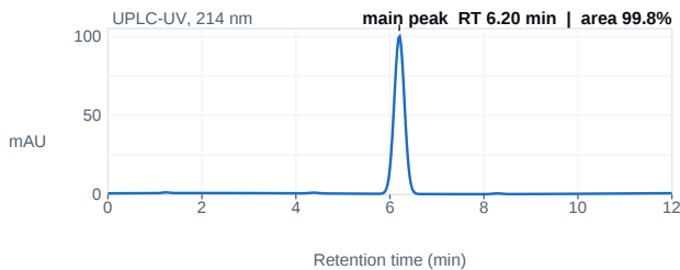
Fig. 1 — UPLC chromatogram; main peak 6.20 min, 99.8% area.
