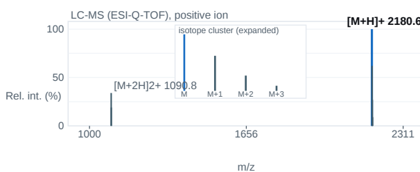
Fig. 2 — ESI-Q-TOF mass spectrum; base peak [M+H] + 2180.6 m/z.
