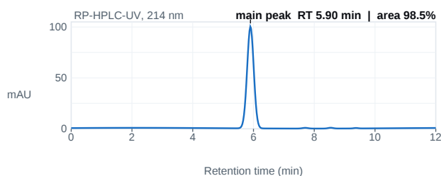
Fig. 1 — HPLC chromatogram; main peak 5.90 min, 98.5% area.
