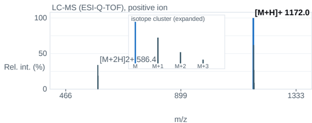
Fig. 2 — ESI-Q-TOF mass spectrum; base peak [M+H] + 1172.0 m/z.
