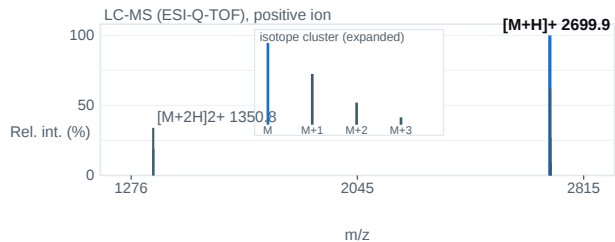
Fig. 2 — ESI-Q-TOF mass spectrum; base peak [M+H] + 2699.9 m/z.
