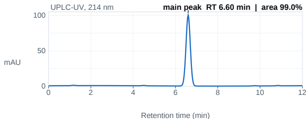
Fig. 1 — UPLC chromatogram; main peak 6.60 min, 99.0% area.
